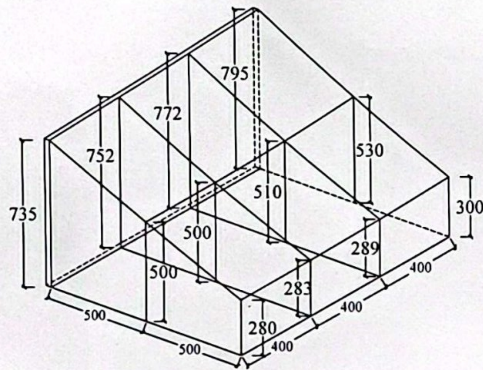
Frame No.53 Quantity- 02 nos (Port & Stbd.)
