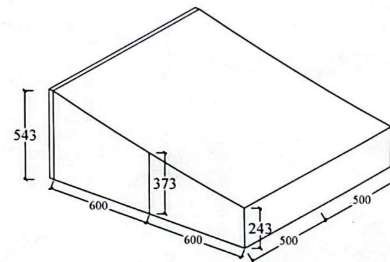
Frame No.116 Quantity- 02 nos (Port & Stbd.)
