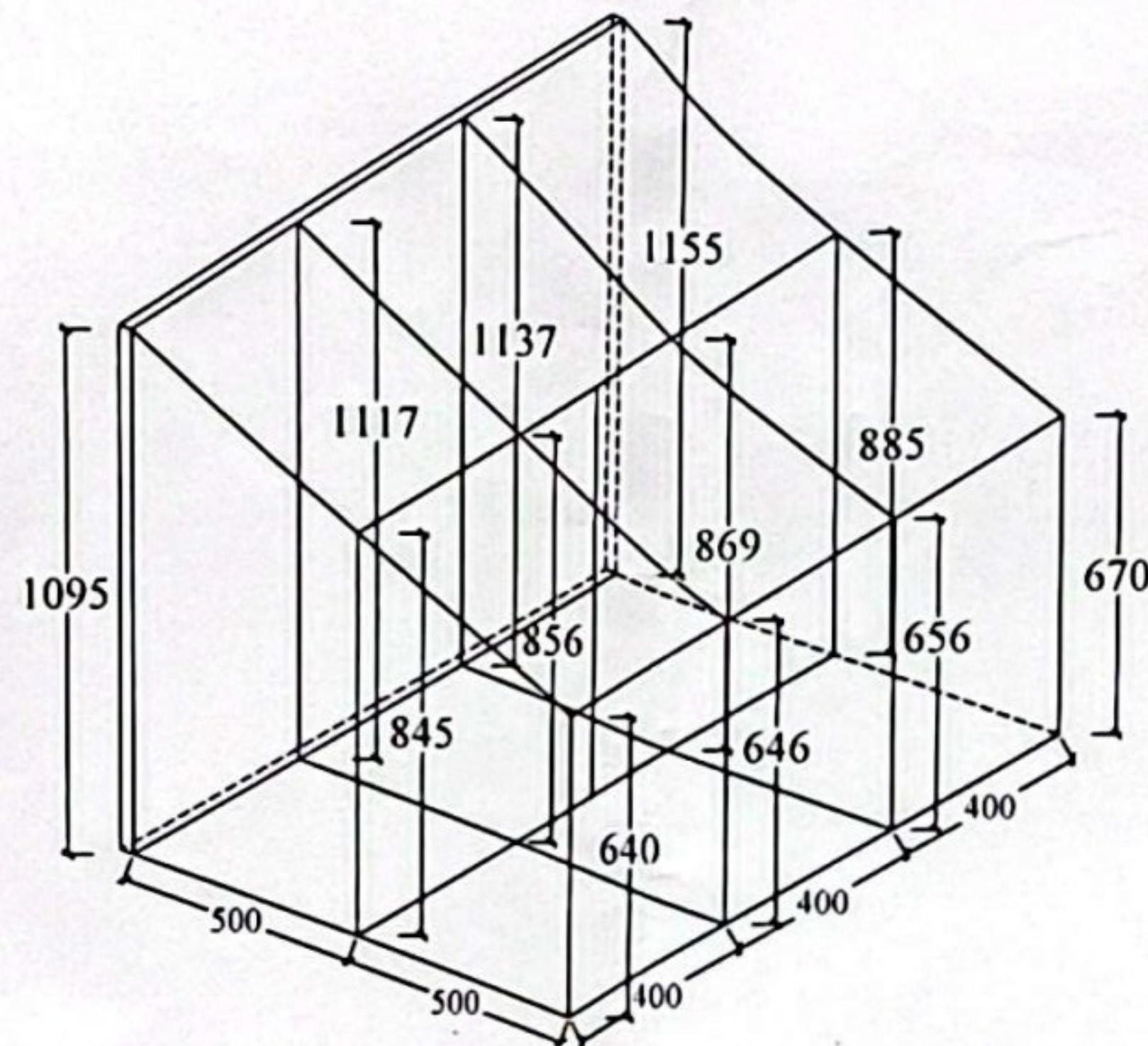
Frame No.72 Quantity- 02 nos (Port & Stbd.)
