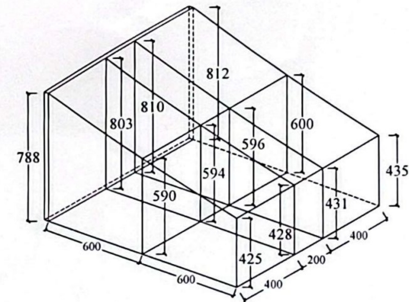
Frame No.91 Quantity- 02 nos (Port & Stbd.)
