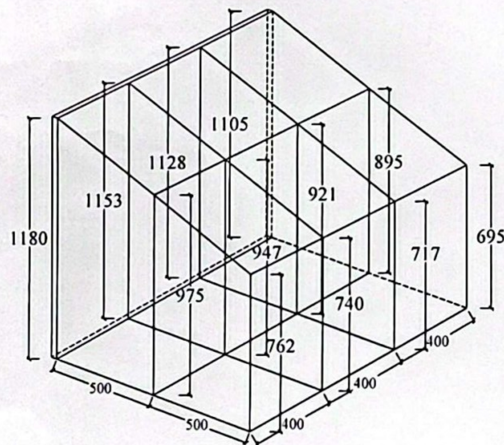
Frame No.148 Quantity- 02 nos (Port & Stbd.)
