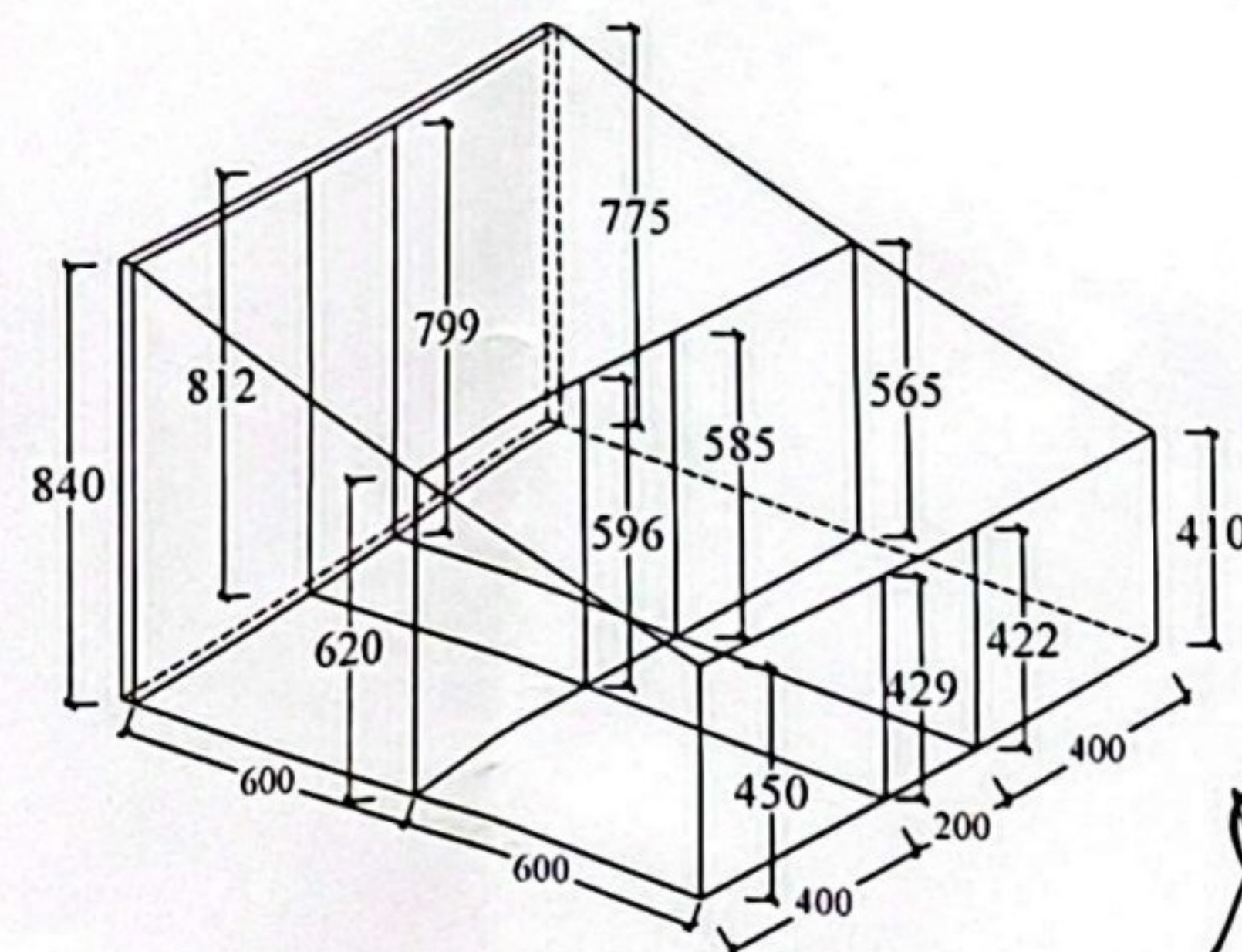
Frame No.133 Quantity- 02 nos (Port & Stbd.)
